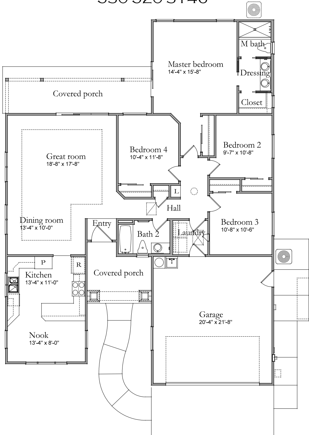
PLAN 1 - ELEVATION A - 4BR/2 BA - 1707 SF
