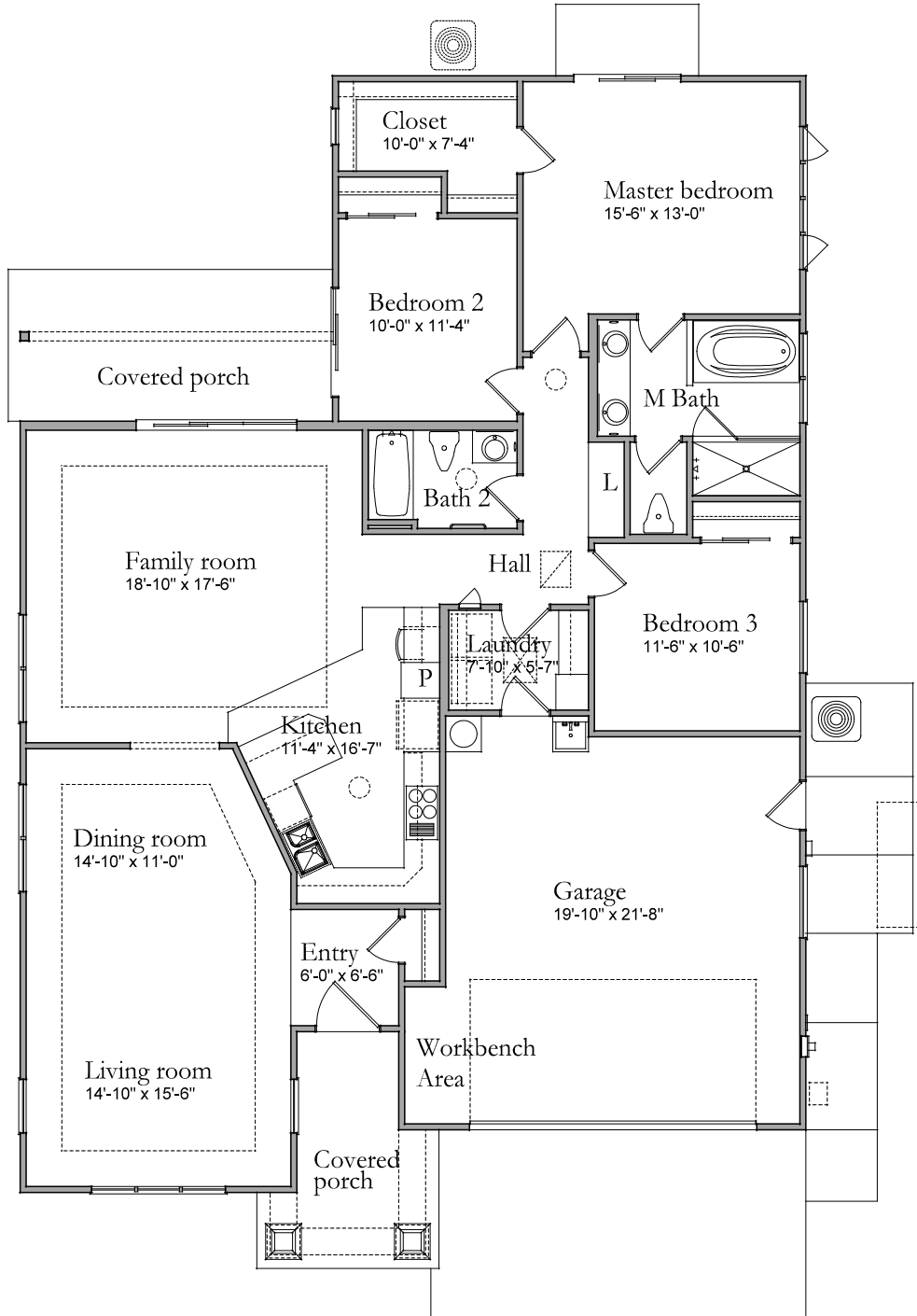
PLAN 2 – ELEVATION A - 3BR/2 BA - 1804 SF
