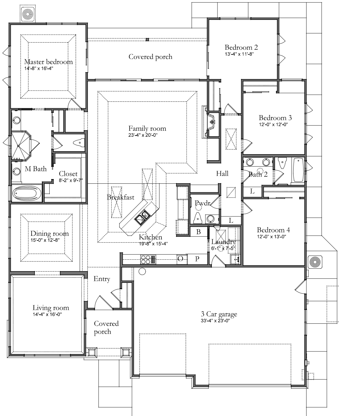
PLAN 9 - ELEVATION A - 4BR/2.5 BA - 2795 SF
