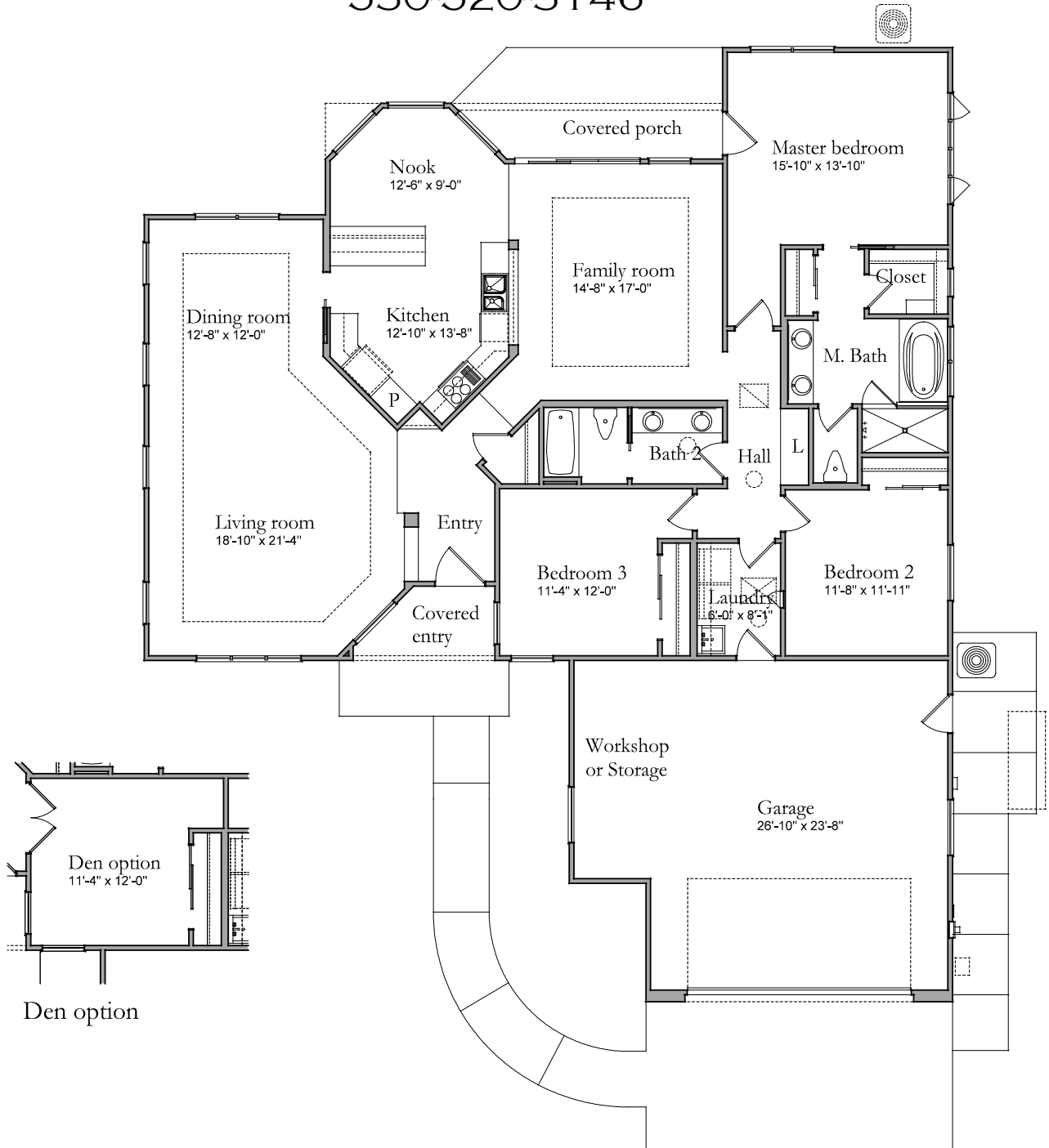
PLAN 5 – ELEVATION C - 3BR/2 BA - 2169 SF
