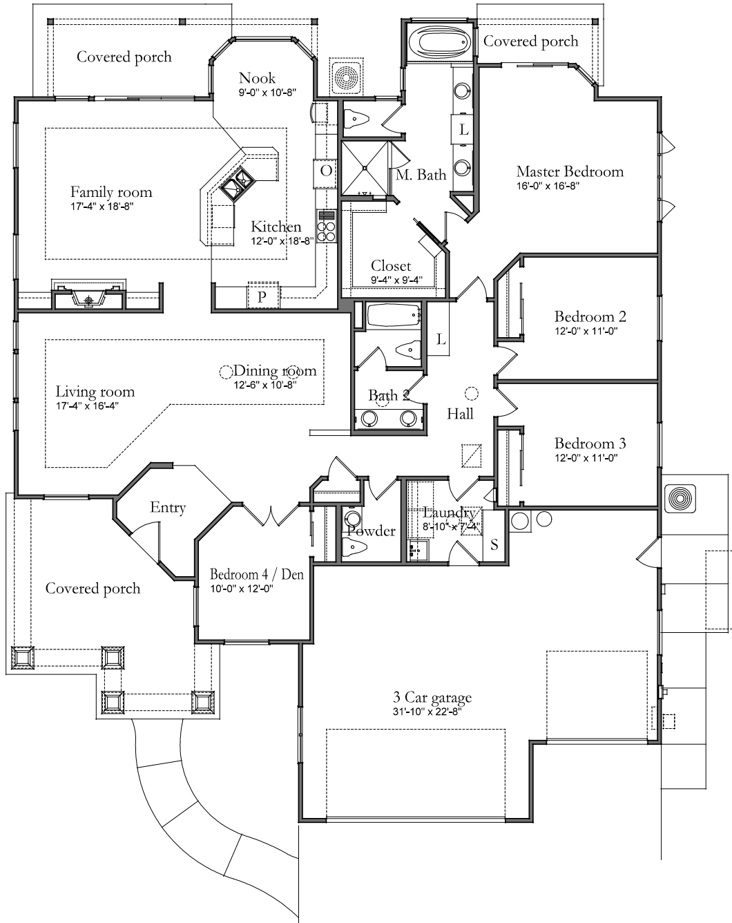
PLAN 8 – ELEVATION B - 4BR/2.5 BA - 2509 SF
