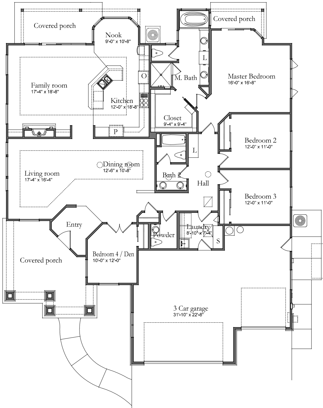
PLAN 8 – ELEVATION C - 4BR/2.5 BA - 2509 SF
