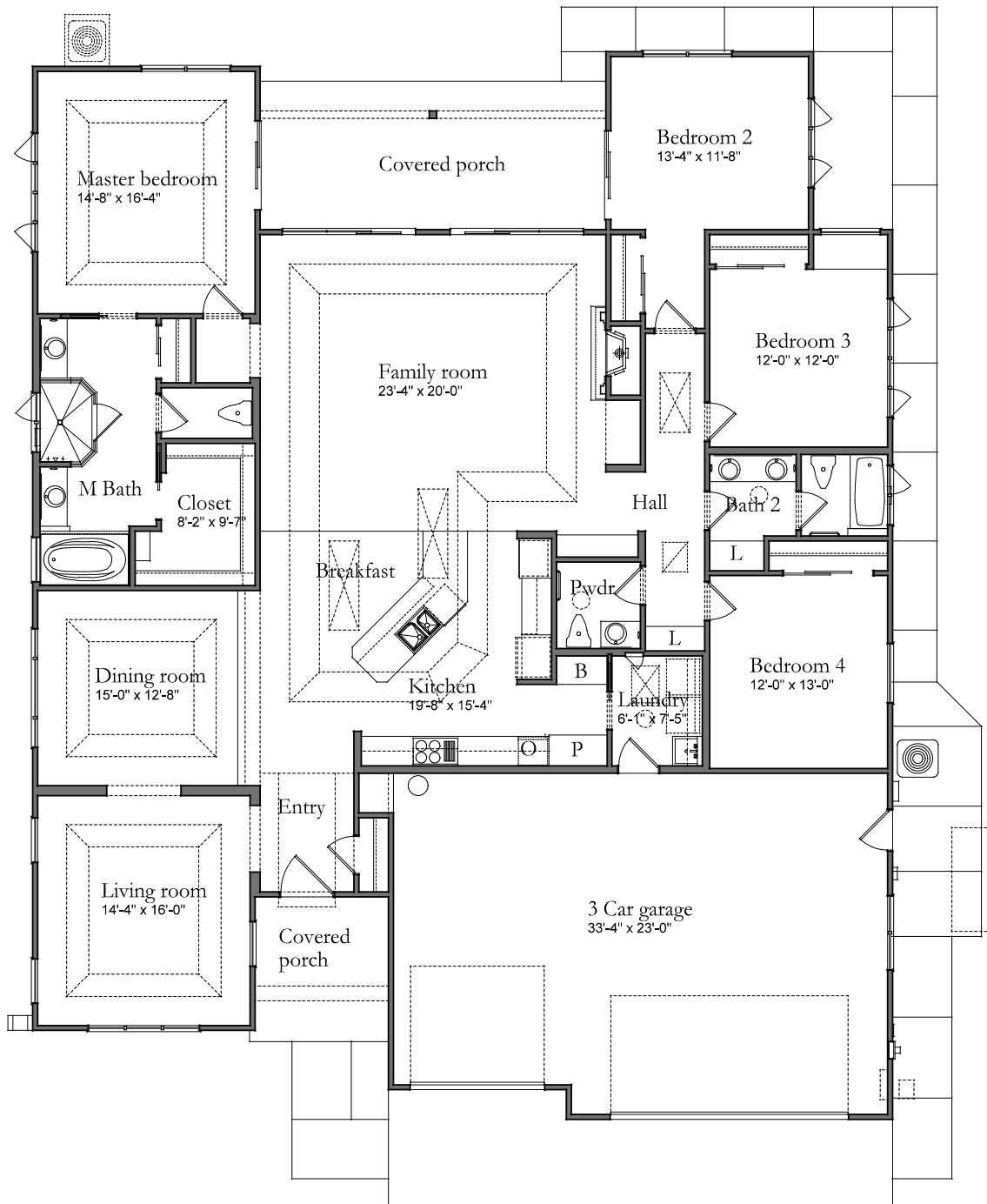
PLAN 9 - ELEVATION C - 4BR/2.5 BA - 2795 SF
