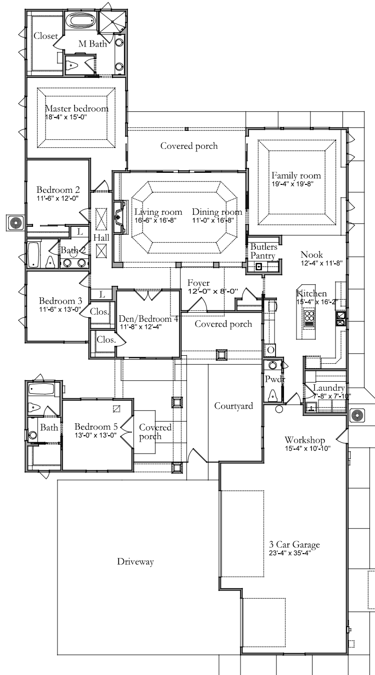
PLAN 10 – ELEVATION B - 5BR/3.5 BA - 3107 SF
